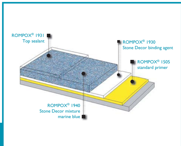
System set up of ROMPOX® Stone Decor, for example 1940 – marine blue
