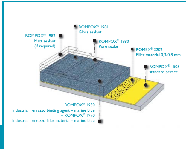
System set up of ROMPOX® Industrial Terrazzo for example 1950 – marine blue
